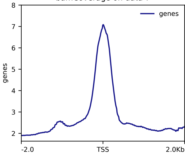
bamCoverage on data 7
